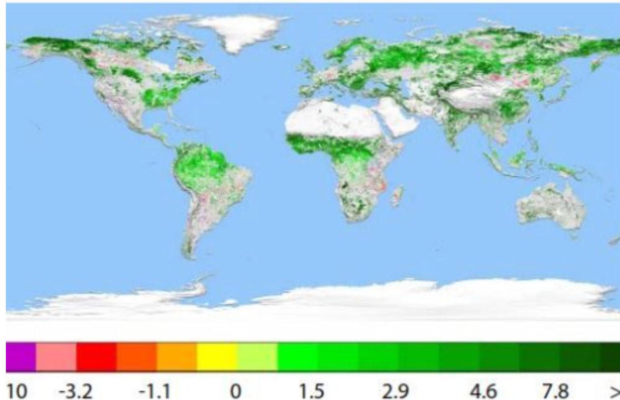
Figure 2: Greening of the Earth, 1982–2011
